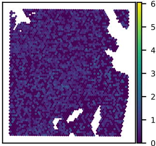
SNU51A LYRM2 expression Moran's I = 0.03
