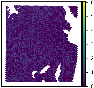
SNU51A PDGFC expression Moran's I = 0.01
