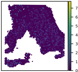
SNU18A ADGRF5 expression Moran's I = 0.05
