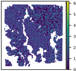
SNU16B TMEM50A expression Moran's I = 0.01
