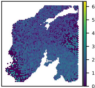
SNU24A HIST1H4H expression Moran's I = 0.20
