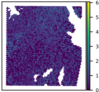
SNU51A TMBIM1 expression Moran's I = 0.08
