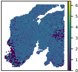
SNU24A EMC10 expression Moran's I = 0.21
