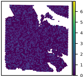
SNU24B SLC18B1 expression Moran's I = 0.03
