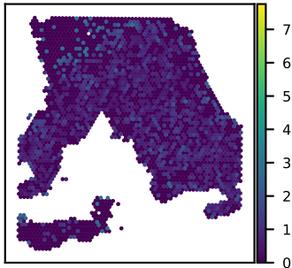
SNU18A TM4SF1 expression Moran's I = 0.07
