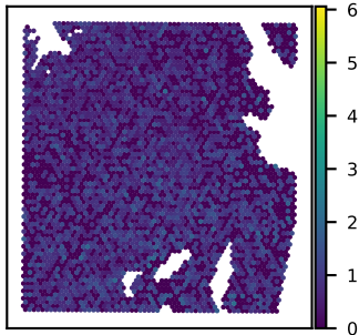
SNU51A SCAMP3 expression Moran's I = 0.03
