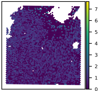
SNU21B SMARCA4 expression Moran's I = 0.10
