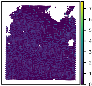
SNU21B NAA35 expression Moran's I = 0.05
