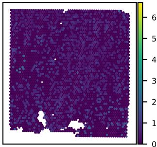
SNU43A RICTOR expression Moran's I = 0.01
