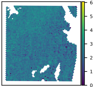
SNU51A PABPC1 expression Moran's I = 0.19
