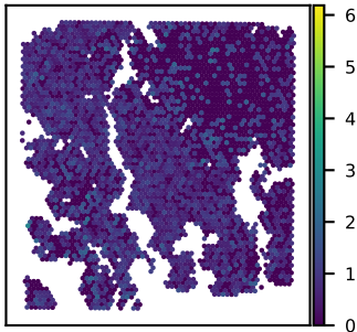
SNU16B TBC1D3B expression Moran's I = 0.08
