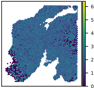
SNU24A TXNL4A expression Moran's I = 0.14
