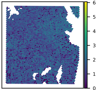
SNU51A G3BP2 expression Moran's I = 0.09
