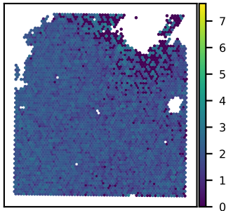
SNU21B COX6C expression Moran's I = 0.15
