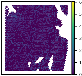
SNU51A THBS2 expression Moran's I = 0.03
