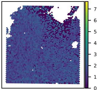
SNU21B ATP5F1A expression Moran's I = 0.12
