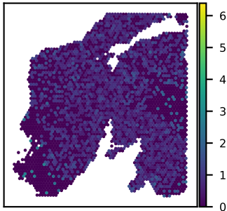
SNU24A WDR35 expression Moran's I = 0.03
