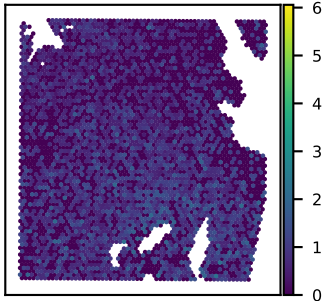
SNU51A C11orf95 expression Moran's I = 0.10
