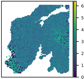
SNU24A SNRNP70 expression Moran's I = 0.02
