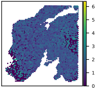
SNU24A TMEM9B expression Moran's I = 0.09
