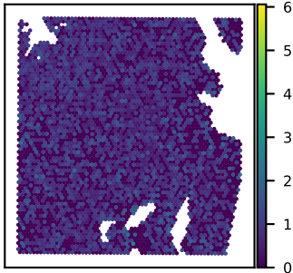
SNU51A TMEM208 expression Moran's I = 0.02
