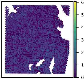
SNU51A YEATS2 expression Moran's I = 0.03
