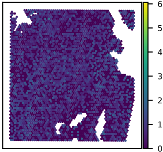
SNU51A ADGRL3 expression Moran's I = 0.02
