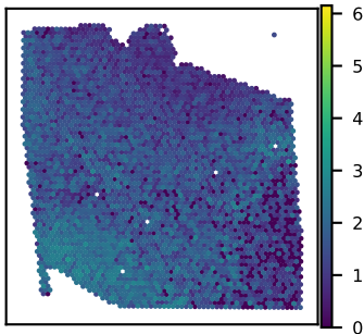
SNU27A DBNDD2 expression Moran's I = 0.35
