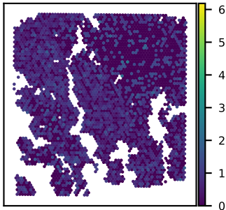
SNU16B TMEM101 expression Moran's I = 0.05
