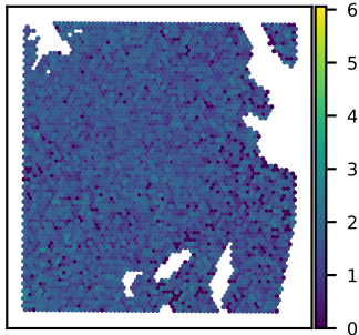
SNU51A C1orf43 expression Moran's I = 0.04
