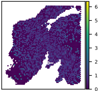
SNU24A ORC3 expression Moran's I = 0.06
