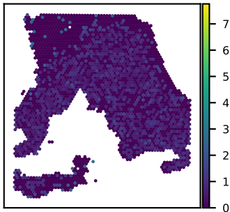
SNU18A SAP30L expression Moran's I = 0.05
