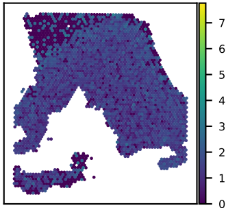
SNU18A COPB2 expression Moran's I = 0.15
