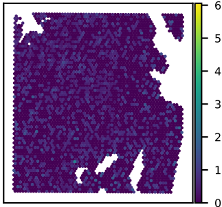
SNU51A THAP3 expression Moran's I = 0.01
