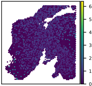
SNU24A EMILIN2 expression Moran's I = 0.05
