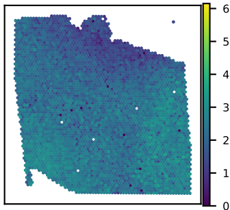
SNU27A MTURN expression Moran's I = 0.56
