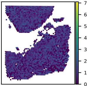
SNU25A SNRPC expression Moran's I = 0.05
