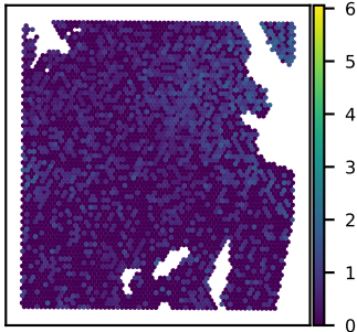
SNU51A RAPGEF4 expression Moran's I = 0.14
