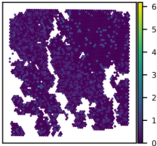
SNU16B PCDHB14 expression Moran's I = 0.02
