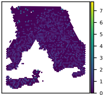
SNU18A SPECC1L expression Moran's I = 0.04
