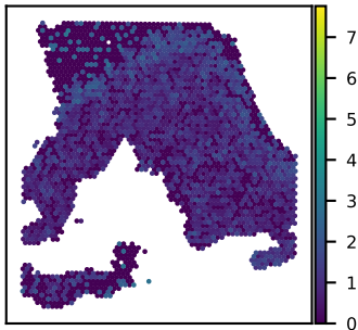
SNU18A PPFIBP1 expression Moran's I = 0.17
