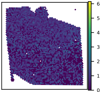
SNU27A HIPK3 expression Moran's I = 0.03
