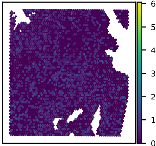
SNU51A DCLRE1B expression Moran's I = 0.03
