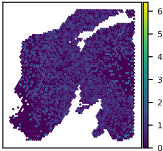
SNU24A EVI5L expression Moran's I = 0.03
