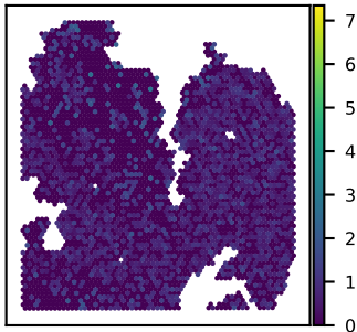
SNU27B C6orf226 expression Moran's I = 0.02
