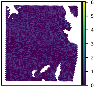
SNU51A ROCK2 expression Moran's I = 0.04
