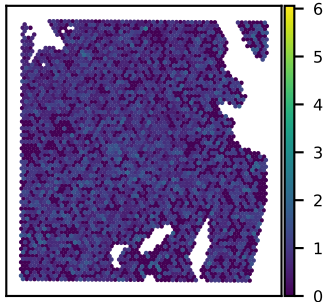
SNU51A NT5C3B expression Moran's I = 0.01
