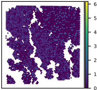
SNU16B KCTD6 expression Moran's I = 0.05
