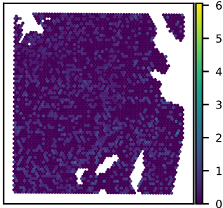
SNU51A CCDC112 expression Moran's I = 0.02
