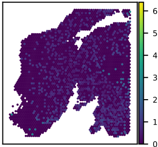
SNU24A CAMKV expression Moran's I = 0.05
